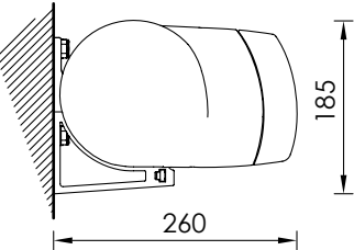
Montaggio a parete Wall installation
